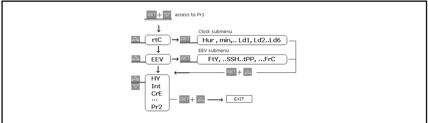
Figure 9-1 - General Structure
