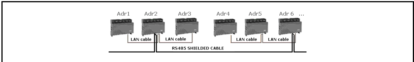
Figure 5-7 - Connecting Monitoring Systems
