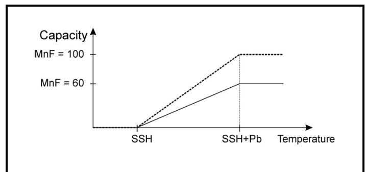
Figure 13-1 - Capacity of Valve in Adjusted MnF Parameter
