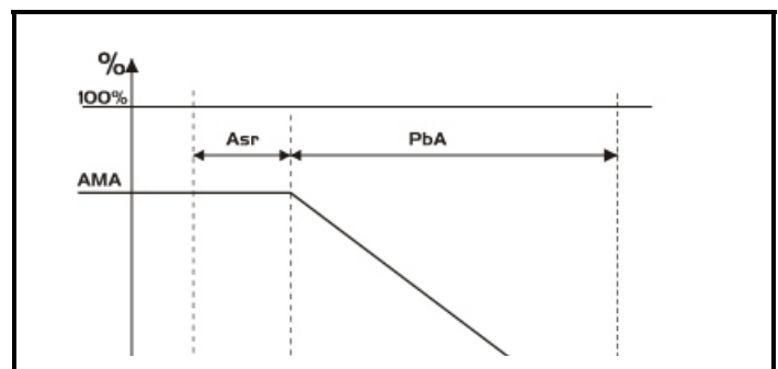
Figure 16-3 - Anti-Sweat Heaters
