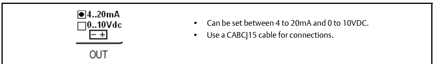
Figure 5-9 - Analog Output
