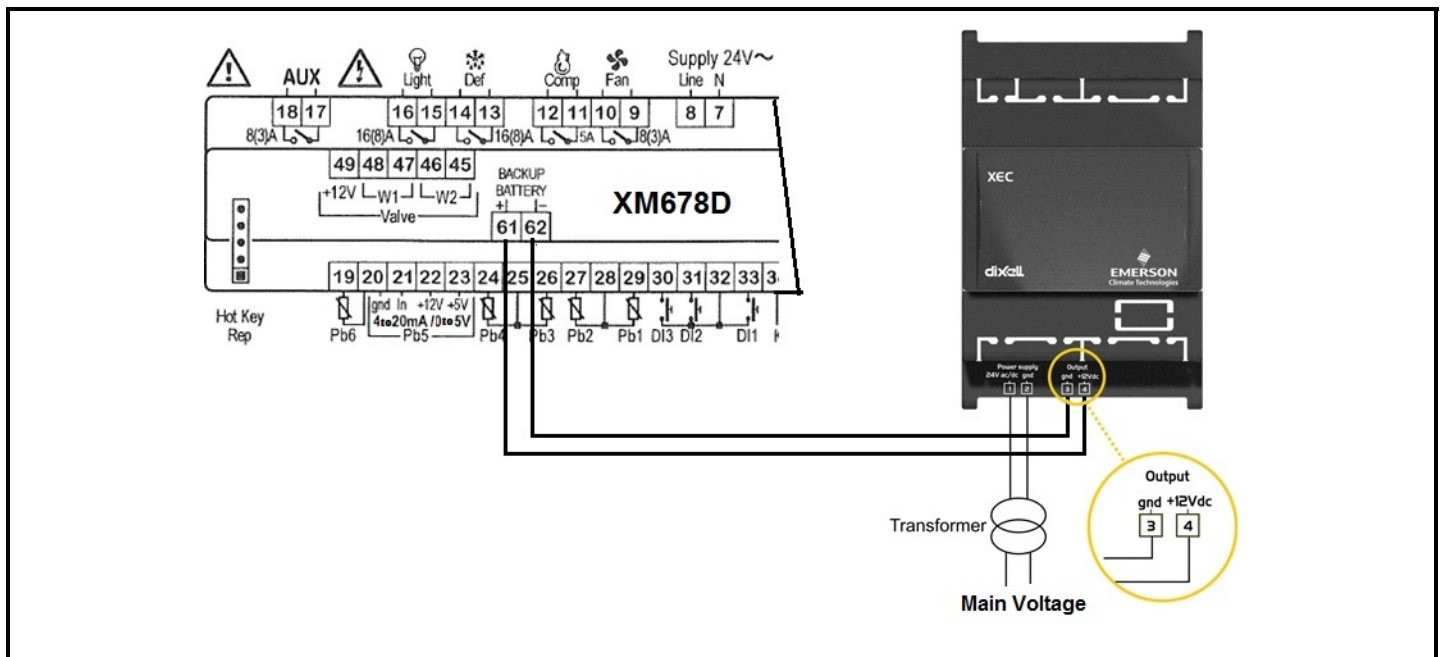
Figure 7-1 - XEC Supercap Connection
