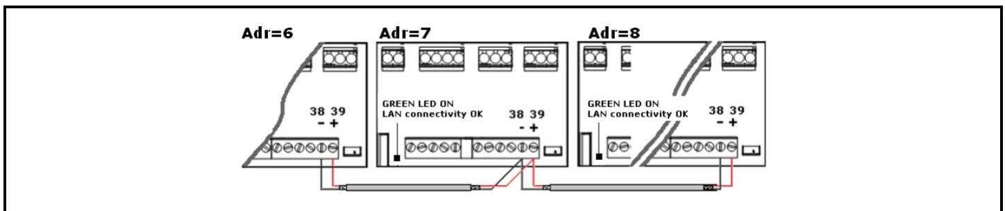
Figure 5-3 - LAN Connection
