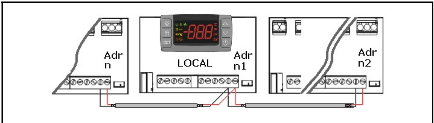
Figure 11-1 - LAN Connection
