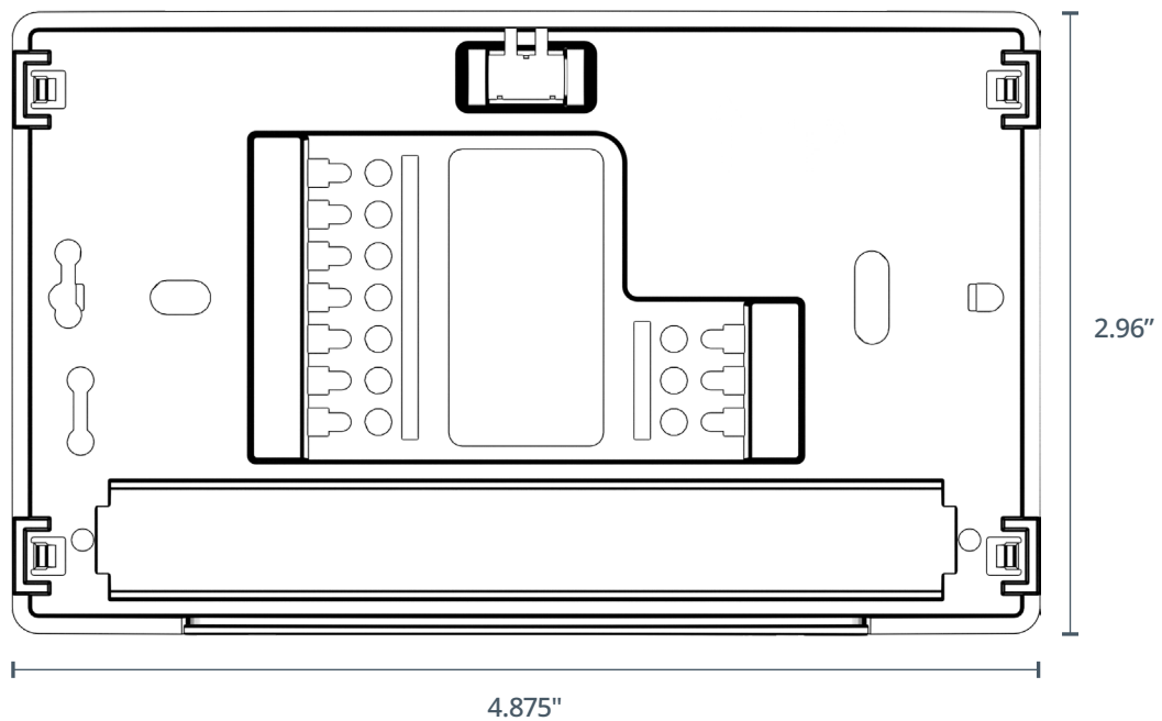
Thermostat backplate
